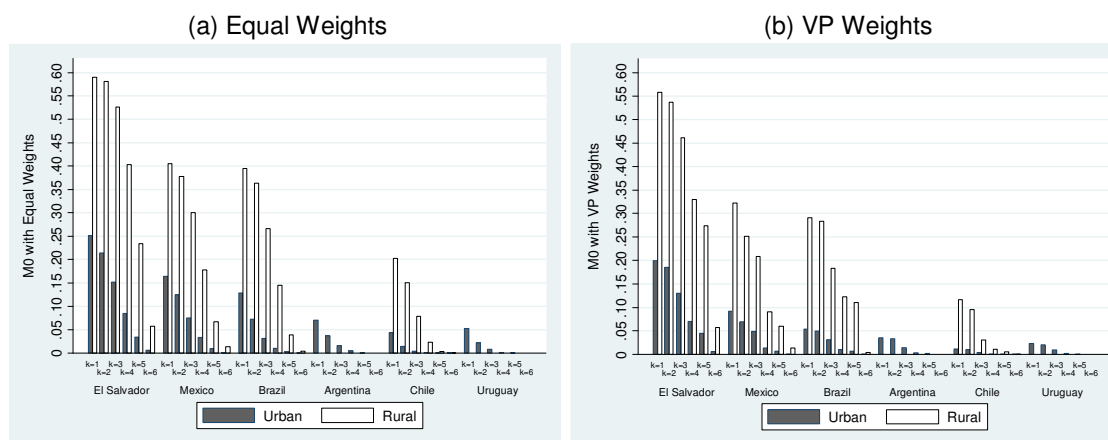
Figure 3: M_0 measure for different k values in 2006 Urban vs. rural areas
