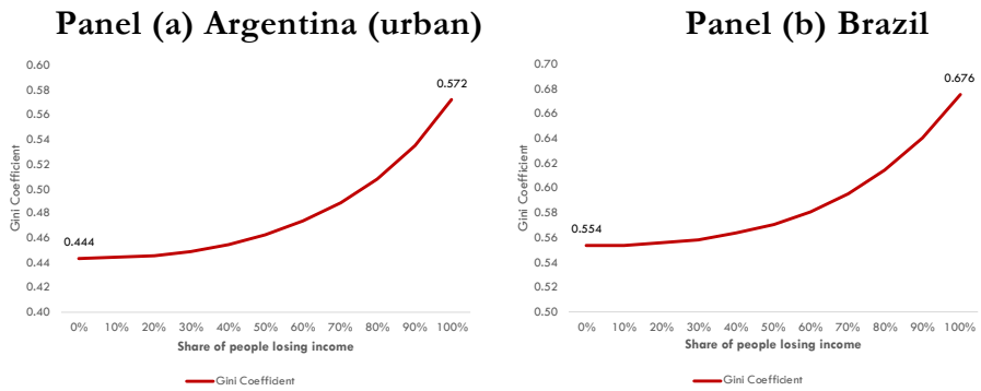
Figure A2. Sensitivity analysis of inequality
