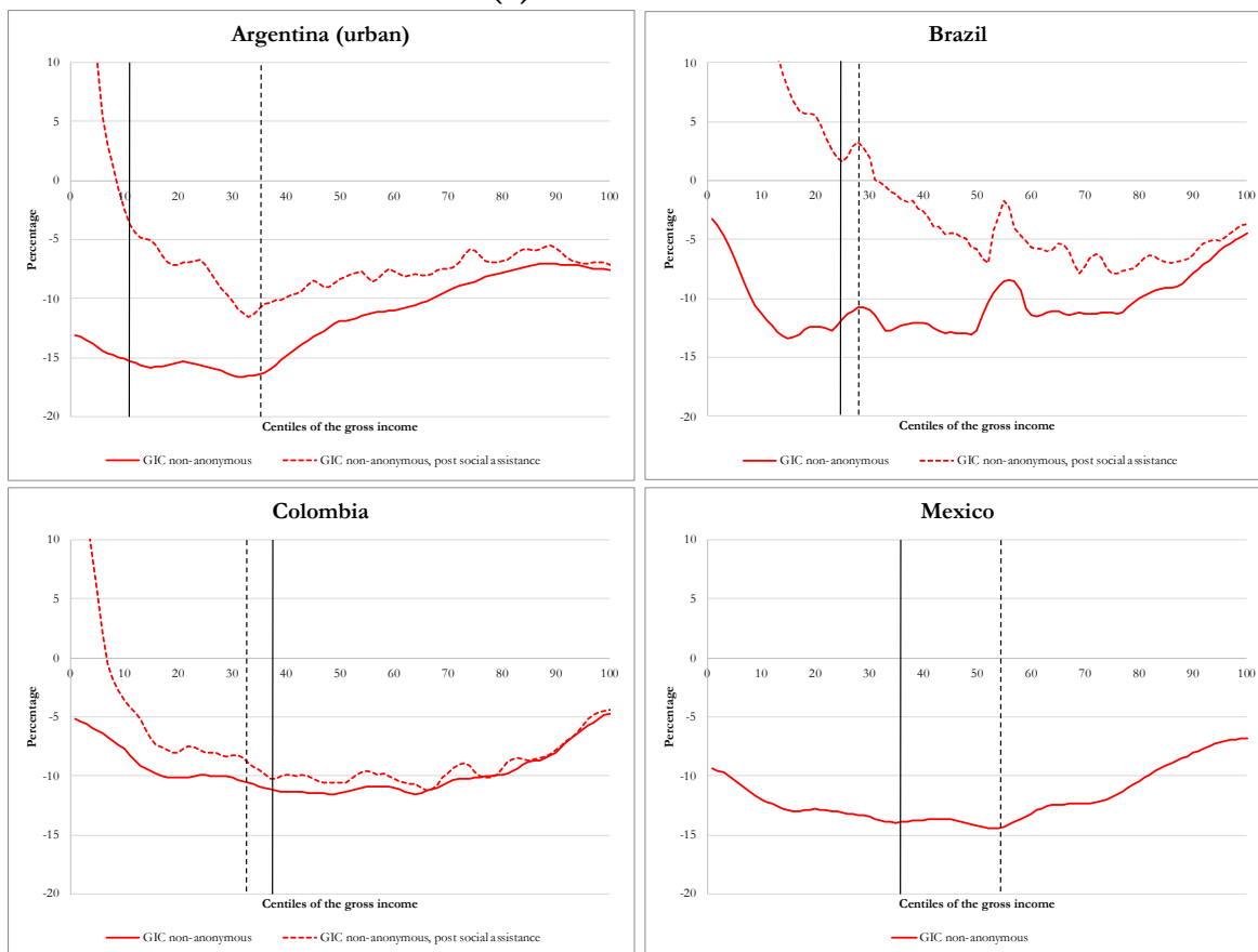
Figure 3. Non-anonymous Growth Incidence Curves Panel (a) “Concentrated losses”
