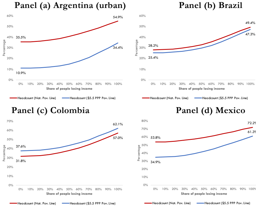
Figure A1. Sensitivity analysis of poverty
