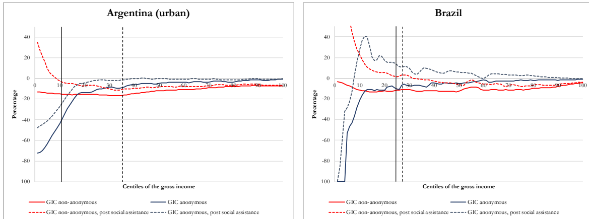
Figure A3. Anonymous and Non-anonymous Growth Incidence Curves Panel (a) “Concentrated losses”
